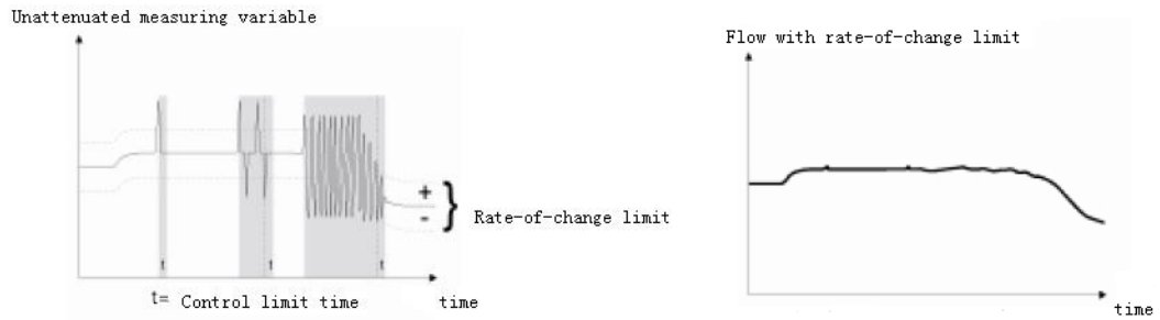
Fig.5 Example for the effect of rate-of-change limit
