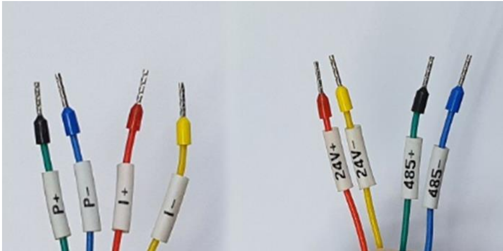
Fig. 3 Cable Connection Identifier
