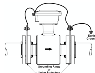
Grounding with Grounding Rings or Lining Protectors
