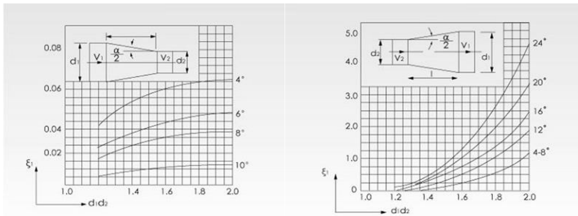
Gradual contraction pipe
